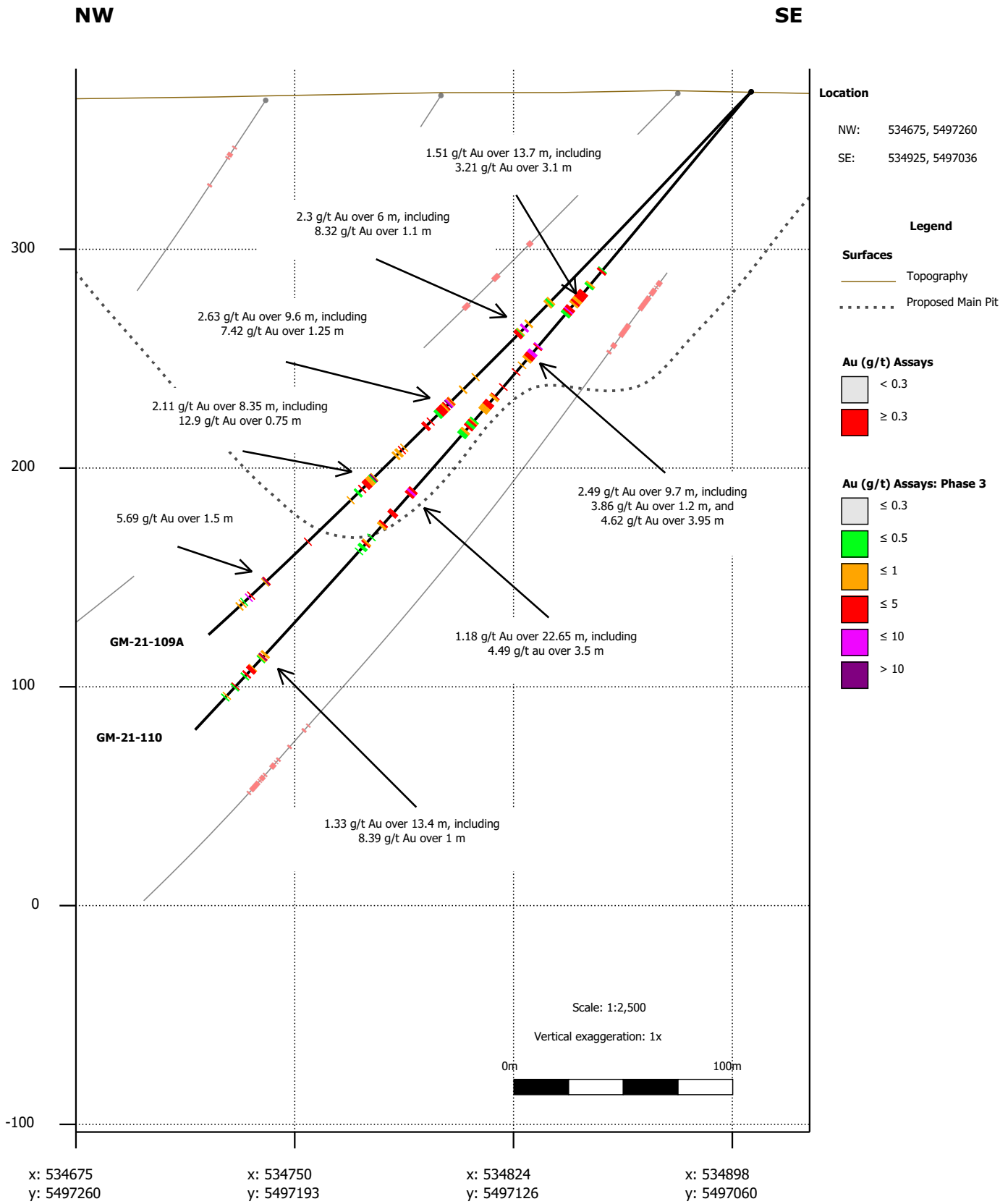
Figure 3: Cross Section - Fox Zone - GM-21-109A + 110 - Chevrier Main Zone Southwest end drill holes (holes clipped up to 10m from section plane)
