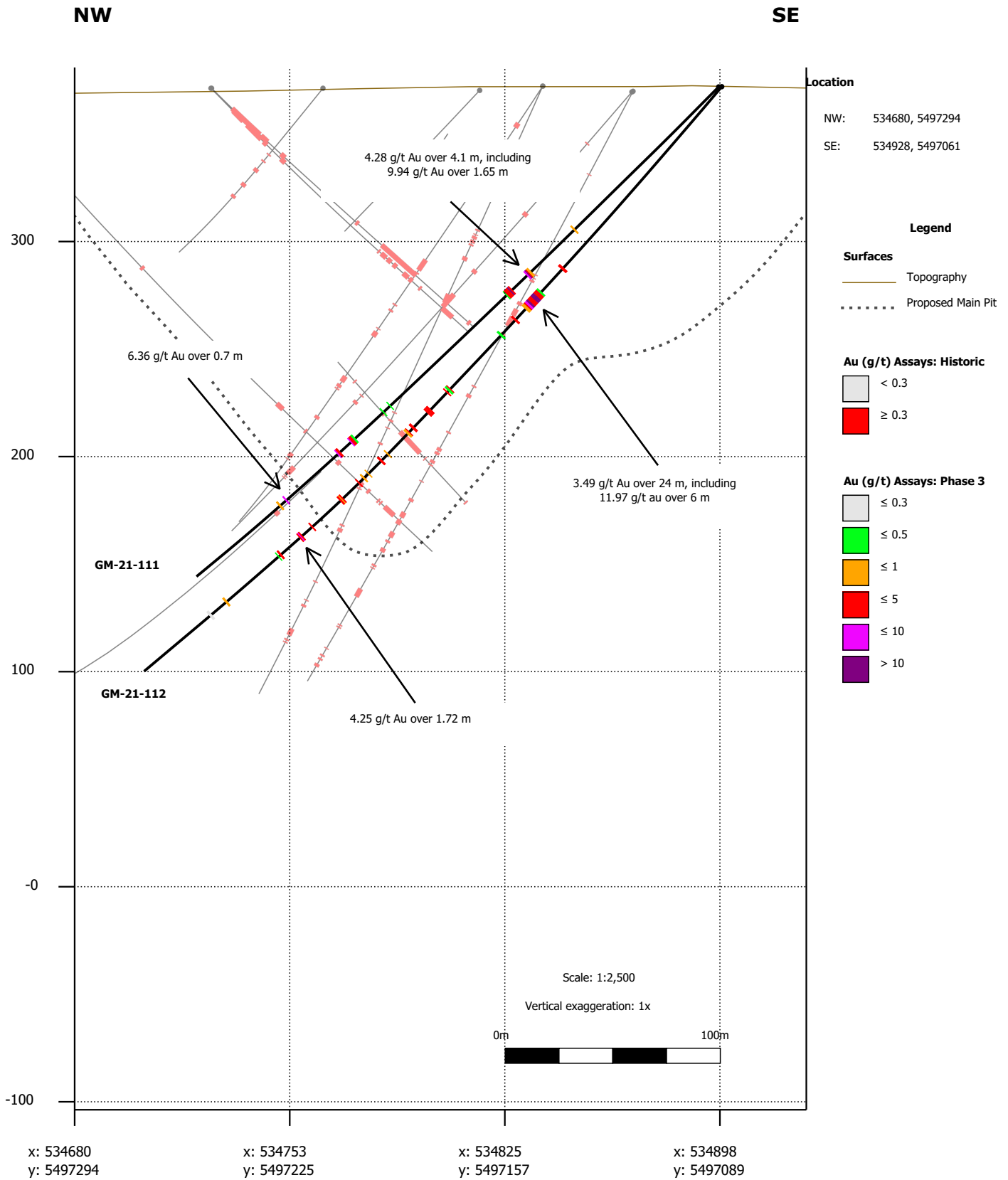
Figure 4: Cross Section - Fox Zone - GM-21-111+112 - Chevrier Main Zone Southwest end drill holes (holes clipped up to 10m from section plane)
